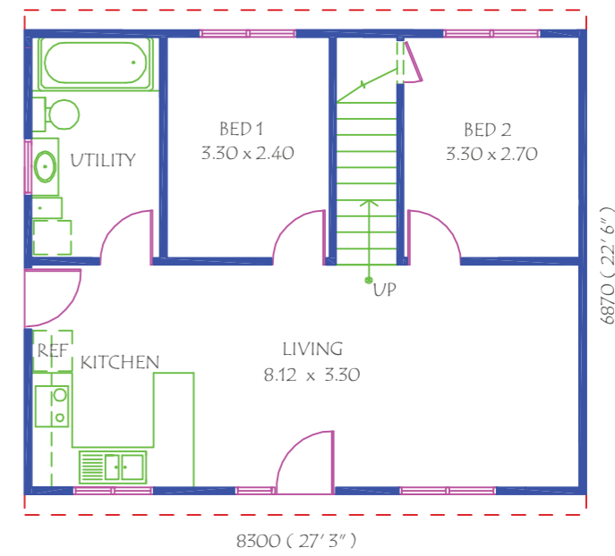
MONTANA ATTIC 3
